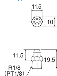
A-PT1/8 type
