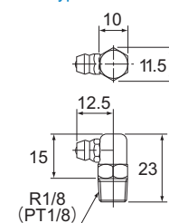
C-PT1/8 type
