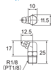
B-PT1/8 type
