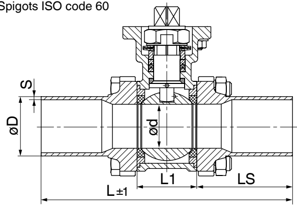
Spigots ISO code 60
