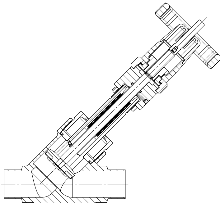
Sectional drawing
